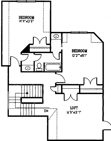
OPTIONAL SECOND FLOOR
